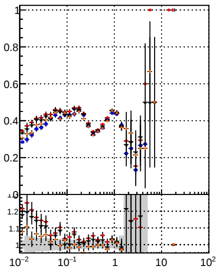
Fake rate vs v Legend: DQM TT MS det0 (blue squares) DQM TT MS det01 (red circles) DQM TT MS det09 (orange crosses) DQM TT MS det09 (black dots)
