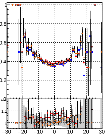
Fake rate vs d BQM MS data BQM MS data
