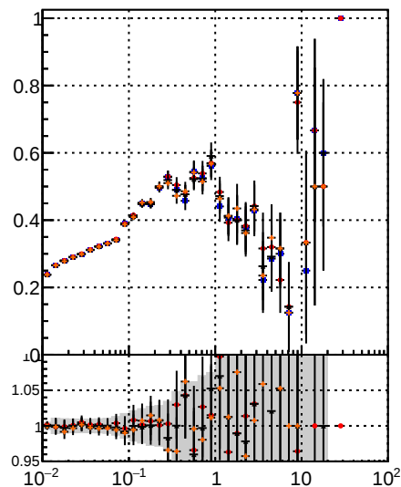
Fake rate vs \nu Legend: DOM TT MS det0 (blue squares), DOM TT MS det01 (red circles), DOM TT MS det09 (orange triangles), DOM TT MS det00 (black crosses)
