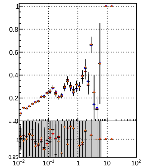
Fake rate vs \nu Legend: DOM TT MS det0 (blue squares) DOM TT MS det01 (red circles) DOM TT MS det09 (orange triangles)
