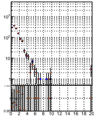
N of associated (recoSim) loopier tracks vs normalized \chi^2
