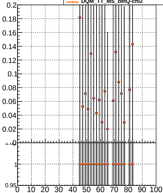
Legend for the bottom row plots: DQM_TT_MS (Blue line with circles) DQM_TT_MS_detQ (Red line with circles) DQM_TT_MS_detQ-dpdq (Black line with circles) DQM_TT_MS_detQ-chi2 (Orange line with circles)
