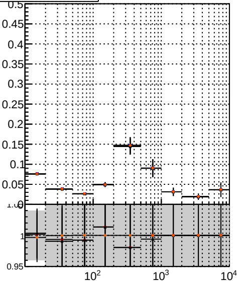
Fakerrate vs Sum p_T^2
