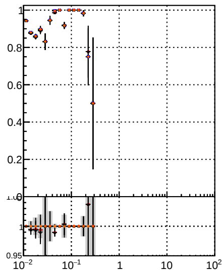
Fake rate vs v Legend: BQM TT MS det0 dndq chiz
