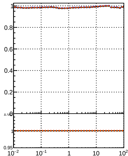
Fake rate vs \sqrt{s} Legend: \text{BQM TT MS det0-dpdq} , \text{BQM TT MS det0-chiz}
