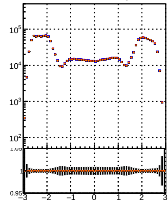
N of reco track vs \eta Legend: BQM (blue line), TT (red line), MS (black line), detQ-dm2d (orange line)
