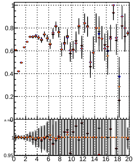
Fake rate vs. Component Blue Square Red Circle Black Triangle DQM TT ~0.8 ~0.8 ~0.8 MS ~0.8 ~0.8 ~0.8 det0 ~0.1 ~0.1 ~0.1 det0-dpda ~0.1 ~0.1 ~0.1 det0-chi2 ~0.1 ~0.1 ~0.1
