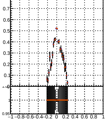
Efficiency vs Dxy(PV)
