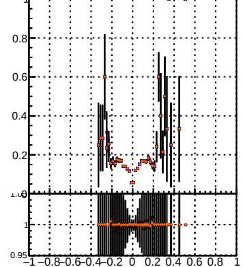
fake+duplicates vs dxy(PV)
