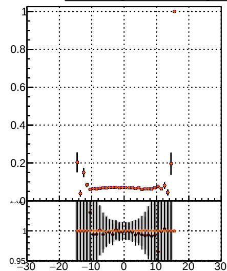
Fake rate vs v Legend: \text{BQM TT MS det0} , \text{BQM TT MS det0-dpdq} , \text{BQM TT MS det0-chiz}
