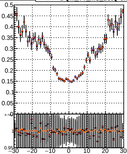
Legend for Fake rate vs v: Blue line: \text{BQM} \rightarrow \text{TT} \rightarrow \text{MS} Red line: \text{BQM} \rightarrow \text{TT} \rightarrow \text{MS} \rightarrow \text{det0-dpdq} Black line: \text{BQM} \rightarrow \text{TT} \rightarrow \text{MS} \rightarrow \text{det0-chiz}
