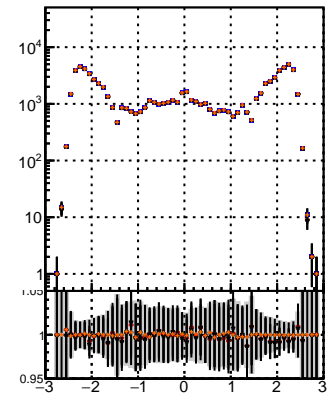
N of reco track vs \eta Legend: BQM (blue), BQM+TT (red), BQM+TT+MS (black), BQM+TT+MS+detQ (orange), BQM+TT+MS+detQ+chir2 (green), BQM+TT+MS+detQ+chir2+chir2 (purple)
