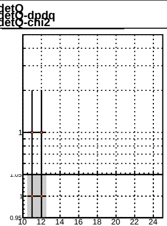
N of associated (recoToSim) tracks vs pixellayer
