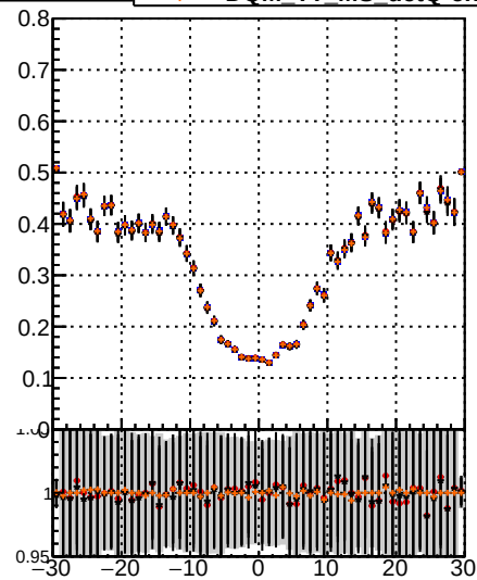
Fake rate vs v Legend: \text{BQM TT MS det0 dndq} , \text{BQM TT MS det0 chiz}
