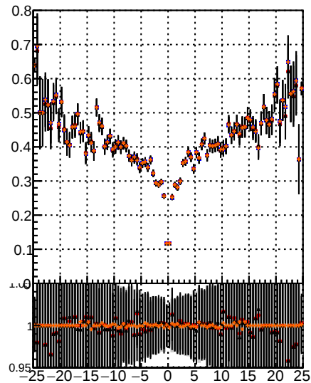
Fake rate vs d MS del18 MS del18-cr12
