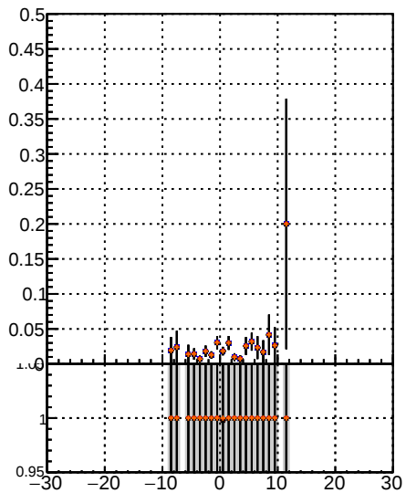
Fake rate vs d Legend: - Blue line: BSM TT MS del8 - Red line: BSM TT MS del8 chr2 - Orange line: BSM TT MS del8 chr2
