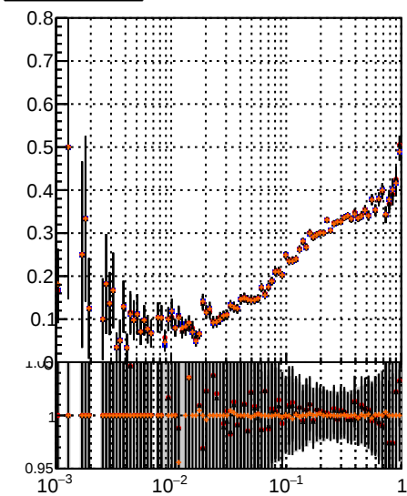
Fake rate vs \text{BQM} \rightarrow \text{TT} \rightarrow \text{MS} \rightarrow \text{det0}
