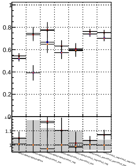
Fake rate vs. —●— BQM IT MS del18 —●— BQM IT MS del19 —●— BQM IT MS del20 —●— BQM IT MS del21 —●— BQM IT MS del22
