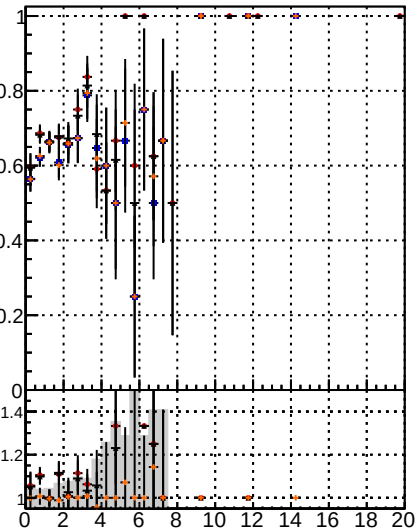
Fake rate vs. —●— BQM IT MS del18 —●— BQM IT MS del19 —●— BQM IT MS del20 —●— BQM IT MS del21 —●— BQM IT MS del22
