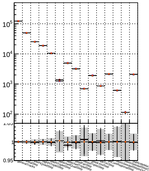
Number of tracks vs collection Legend: Blue line with circles: DQM TT MS Orange line with diamonds: DQM TT MS_detQ Black line with triangles: DQM TT MS_detQ-dpdq Orange line with squares: DQM TT MS_detQ-chi2
