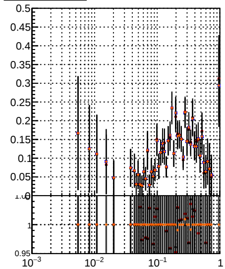
Pileup rate vs \eta
