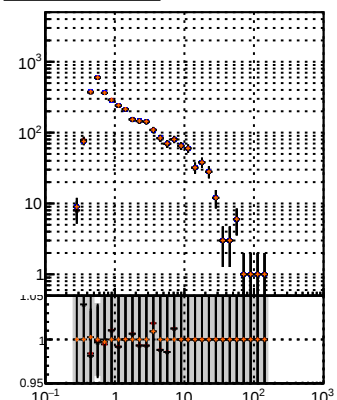
N of reco track vs \eta BQM TT MS detQ-dm2d BQM TT MS detQ-dm2d BQM TT MS detQ-dm2d
