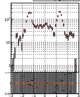
N of reco track vs \eta BQM TT MS detQ-dm2d BQM TT MS detQ-dm2d BQM TT MS detQ-dm2d
