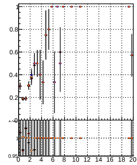
Fake rate vs. BSM MS det18 BSM MS det18
