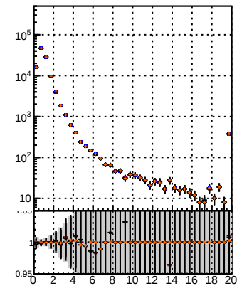
N of associated (recoSim) tracks vs normalized \chi^2
