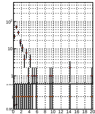
N of associated (recoSim) loop tracks vs normalized \chi^2
