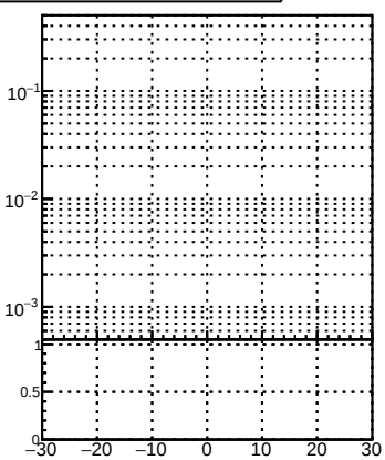
l of associated (recoToSim) looper tracks vs transverse ref point position
