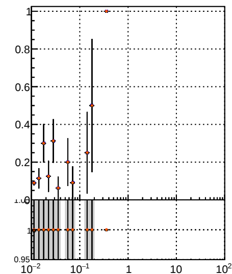
Fake rate vs v_{\text{top}} Legend: \text{BQM TT MS det0 dndq} , \text{BQM TT MS det0 chiz}
