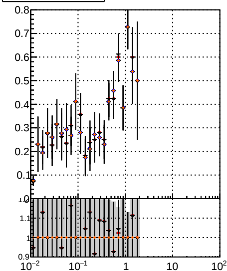
Fake rate vs v_{\text{xy}} Duplicates Rate vs v_{\text{xy}} Pileup rate vs v_{\text{xy}}
