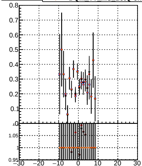
Fake rate vs v_{\text{xy}} Duplicates Rate vs v_{\text{xy}} Pileup rate vs v_{\text{xy}}
