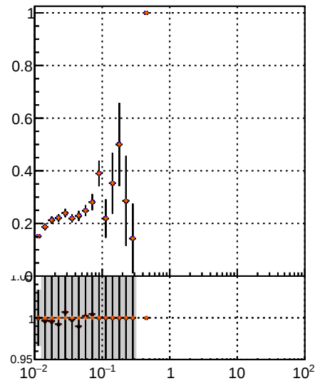
Fake rate vs \sqrt{s} \overline{B}0M TT MS \overline{B}0M TT MS det0 \overline{B}0M TT MS det0-dpdq \overline{B}0M TT MS det0-chiz \overline{B}0M TT MS \overline{B}0M TT MS det0 \overline{B}0M TT MS det0-dpdq \overline{B}0M TT MS det0-chiz
