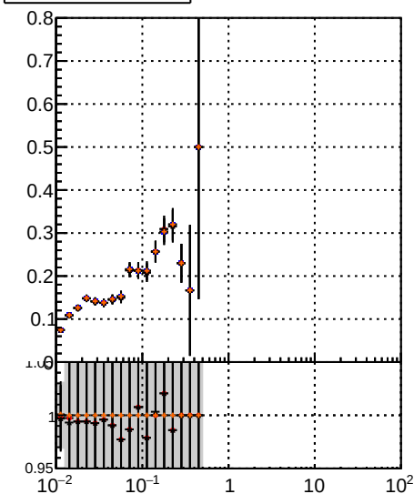
Fake rate vs v — BBM TT MS det0 — BBM TT MS det0-dpdq — BBM TT MS det0-chiz
