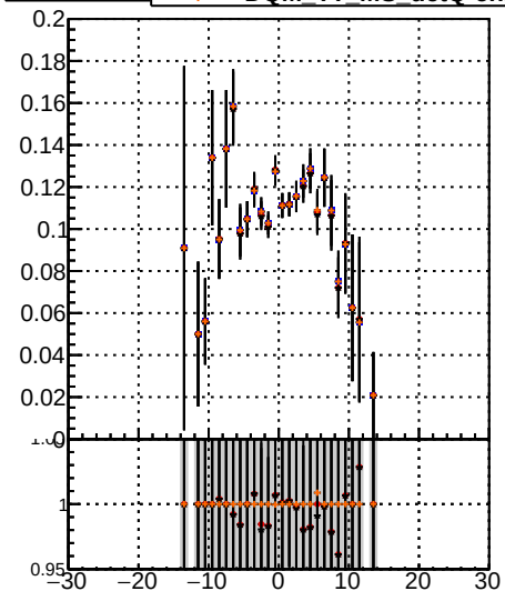
Fake rate vs v — BBM TT MS det0 — BBM TT MS det0-dpdq — BBM TT MS det0-chiz
