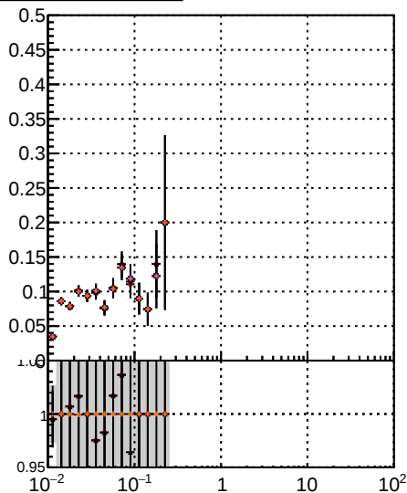
Fake rate vs \sqrt{s} Legend DDM TT MS det0-dpdq det0-chiz Blue line with dots DDM TT MS det0-dpdq det0-chiz Red line with dots DDM TT MS det0-dpdq det0-chiz Black line with dots DDM TT MS det0-dpdq det0-chiz Orange line with dots DDM TT MS det0-dpdq det0-chiz
