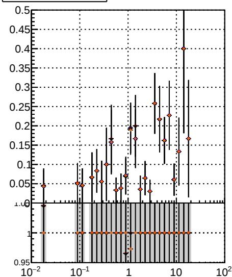
Fake rate vs \sqrt{s} —●— DDM TT MS det0 —●— DDM TT MS det0-dpdq —●— DDM TT MS det0-chiz
