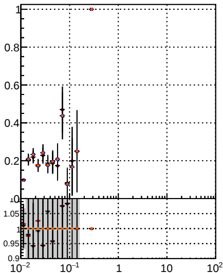
Fake rate vs \sqrt{s} —●— BBM TT MS det0 —●— BBM TT MS det0-dpdq —●— BBM TT MS det0-chiz
