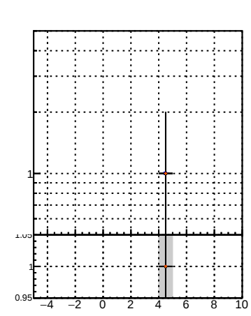
N of associated (recoToSim) loopers tracks vs. sim PV z
