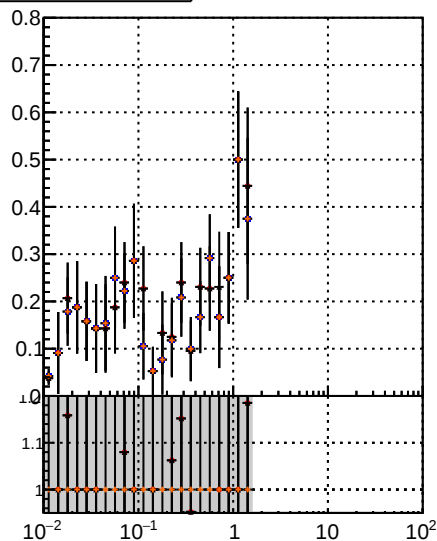
Legend: - \text{BQM} \rightarrow \text{TT} \rightarrow \text{MS} \text{det0-dpdq} - \text{BQM} \rightarrow \text{TT} \rightarrow \text{MS} \text{det0-chiz} - \text{BQM} \rightarrow \text{TT} \rightarrow \text{MS} \text{det0-chiz}
