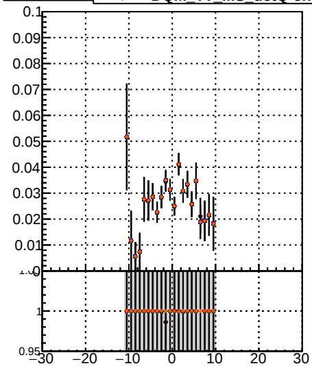
Fake rate vs v Legend: \text{BQM TT MS det0-dpdq} , \text{BQM TT MS det0-chiz}
