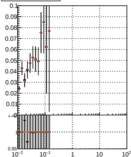
Fake rate vs v Legend: \text{BQM TT MS det0-dpdq} , \text{BQM TT MS det0-chiz}
