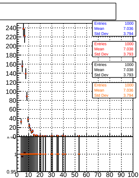
Uncertainty z Coordinate (tagged Vtx)
