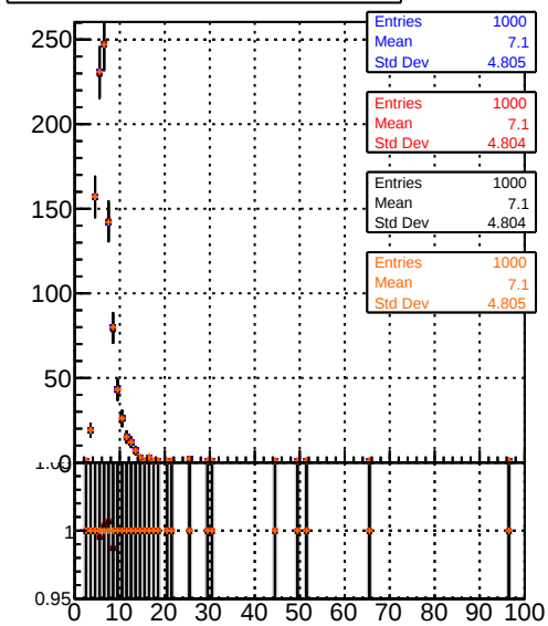
Uncertainty x Coordinate (tagged Vtx)
