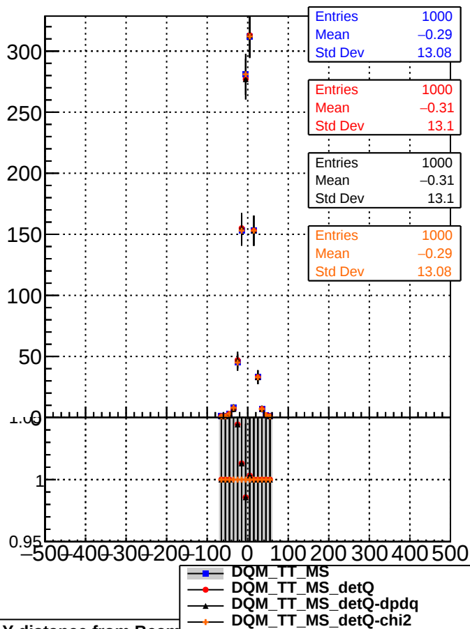
Y distance from BeamSpot (tagged Vtx)
