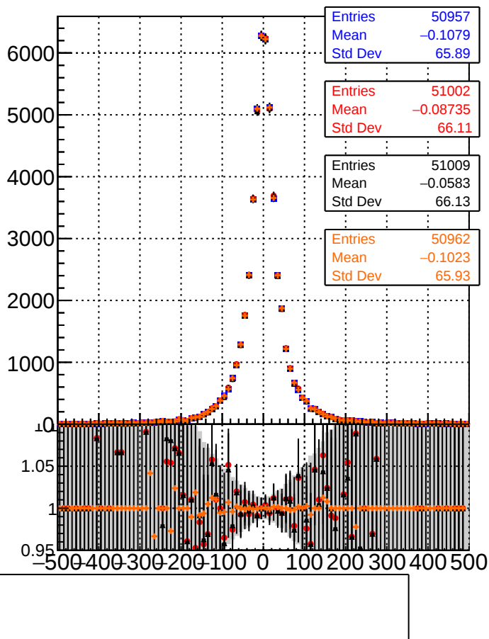
Y distance from BeamSpot (other Vtx)
