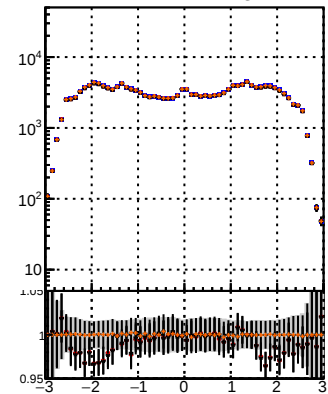
N of reco track vs \eta Legend: BQM (black), TT (red), MS (blue), detQ (orange)
