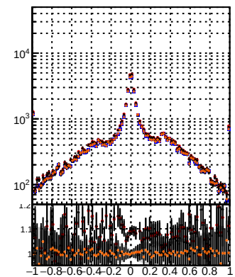
N of reco track vs dxy(PV) det0-dpda det0-chi2 det0-dpda det0-chi2
