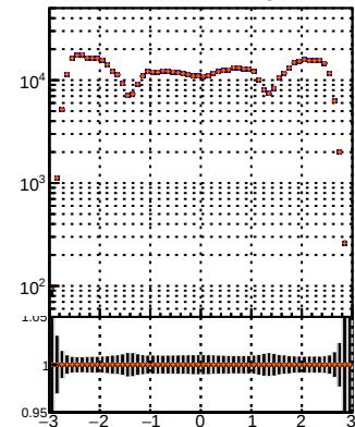
N of reco track vs \eta BQM TT MS det0-dm2d BQM TT MS det0-dm2d BQM TT MS det0-dm2d
