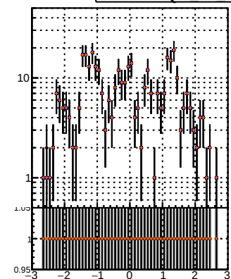
N of reco track vs \eta BQM TT MS detQ BQM TT MS detQ-dm2d
