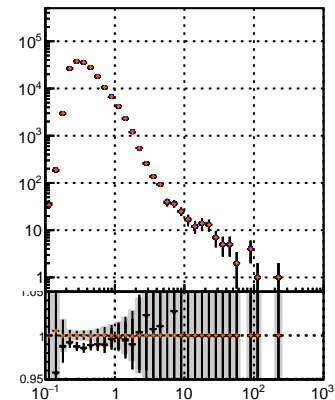
N of reco track vs e DQM TT MS detO detC
