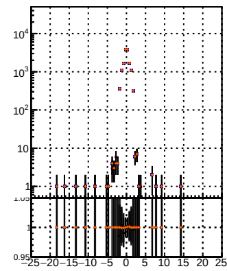
N of reco track vs dxy(PV) vs dxy(PV) DQM TT MS MS det0-dpda det0-dpda det0-chi2
