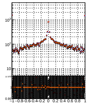
N of reco track vs dxy(PV) vs dxy(PV) DQM TT MS MS det0-dpda det0-dpda det0-chi2
