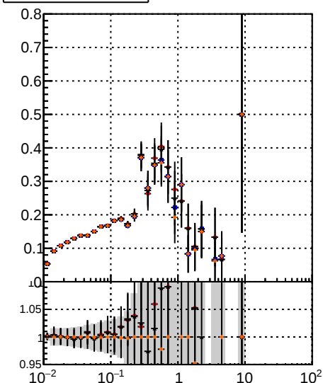
Fake rate vs \nu BQM TT MS det0 BQM TT MS det0-dpdq BQM TT MS det0-chiz BQM TT MS det0-chiz-dpdq
