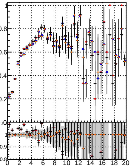
Fake rate vs. DOM TT MS det0 det0-dpda DOM TT MS det0 det0-chi2
