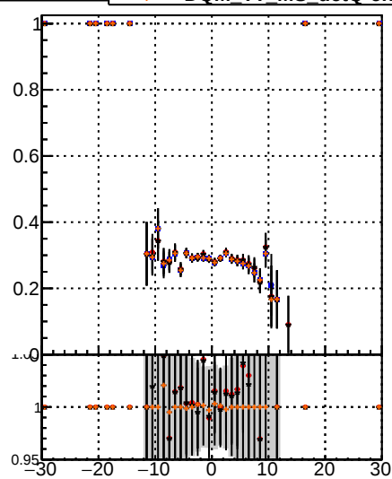
Fake rate vs \nu BQM TT MS det0 dndq BQM TT MS det0-chiz
