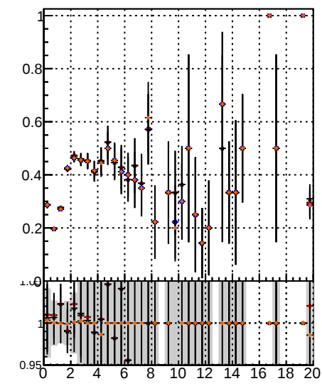
Fake rate vs. BQM MS det18 det24 BQM MS det18 det24
