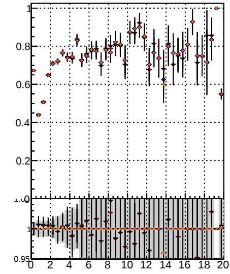
Fake rate vs. \chi^2
